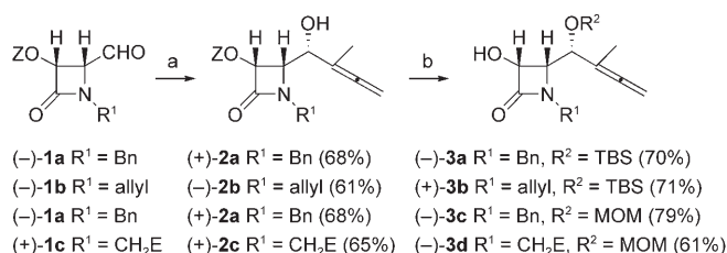
Scheme 1. Synthesis of enantiopure monocyclic \gamma -allenols 3a–d .
